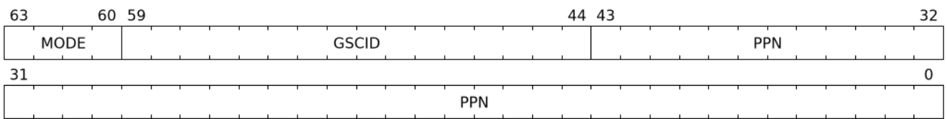
Figure 16. IO hypervisor guest address translation and protection ( iohgap ) field
