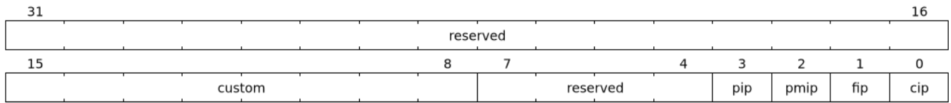
Figure 50. Interrupt pending status register fields
