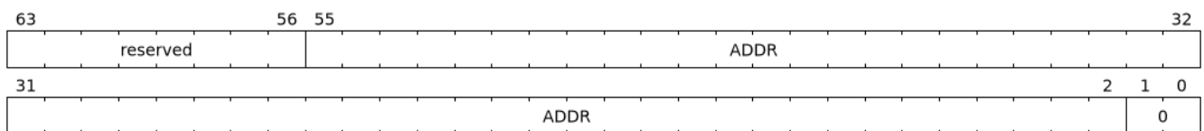
Figure 61. Message address register fields
