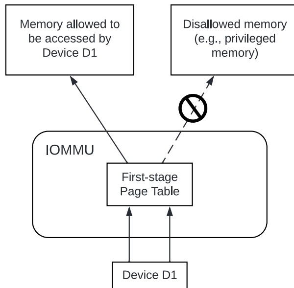
Figure 1. Device isolation in non-virtualized OS
